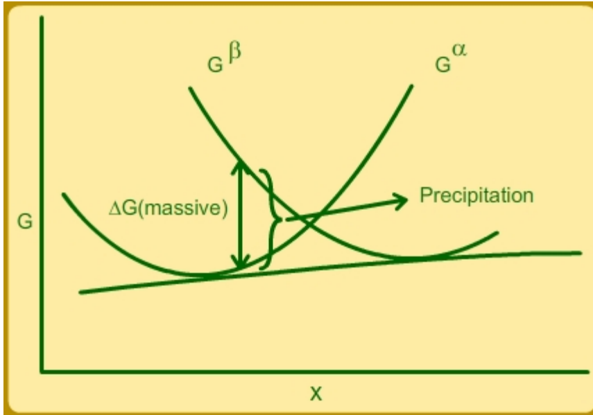
Figure 38: Massive transformation in a two phase region.
