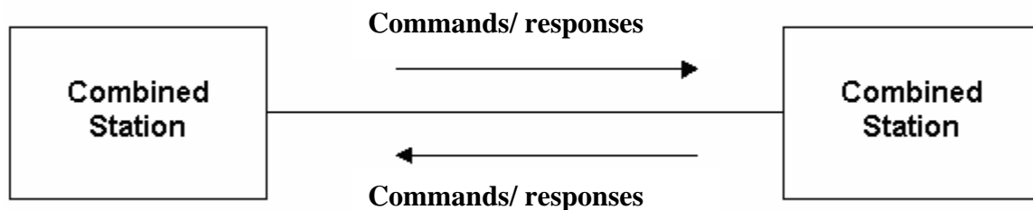
Figure 3.4.2 Balanced configuration
