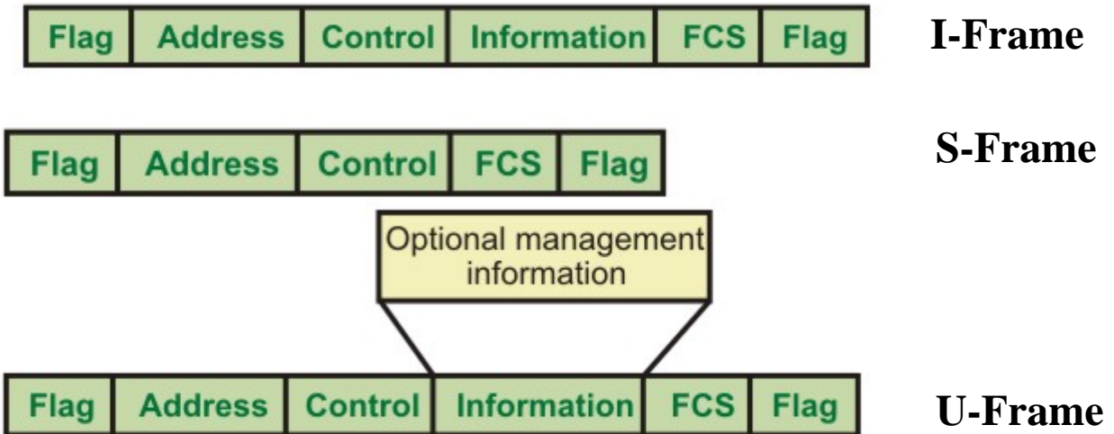
Figure 3.4.4 Different types of frames used in HDLC
