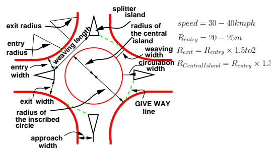
Figure 32:2: Design elements of a rotary
