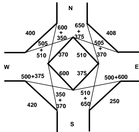
Figure 32:5: Traffic negotiating a rotary
