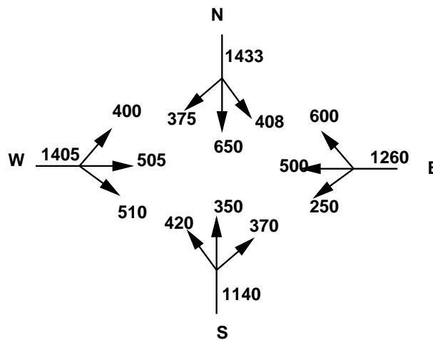
Figure 32:4: Traffic approaching the rotary
