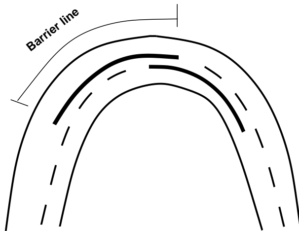
Figure 29:8: No passing zone marking at horizontal curves
