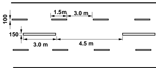
Figure 29:6: Traffic lane marking for a four lane road with broken center line
