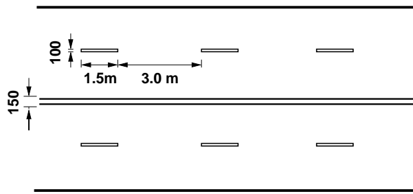
Figure 29:5: Lane marking for a four lane road with solid barrier line
