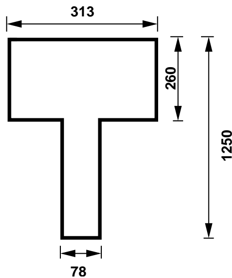
Figure 29:14: Typical dimension of the character T used in road marking
