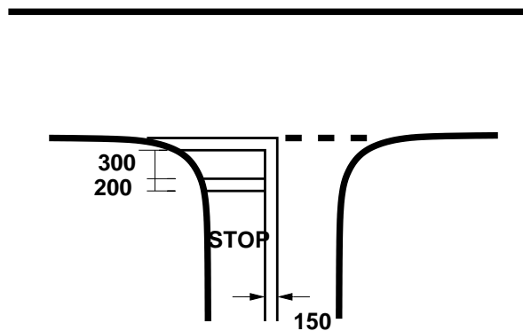
Figure 29:10: Stop line marking near an intersection
