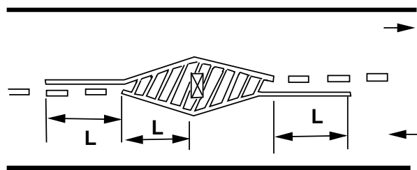
Figure 29:15: Approach marking for obstructions on the road way
