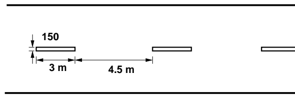
Figure 29:1: Center line marking for a two lane road
