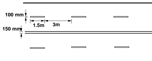
Figure 29:4: Center barrier line marking for four lane road
