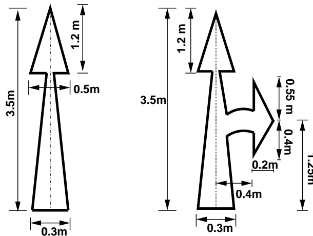
Figure 29:12: Directional arrow marking
