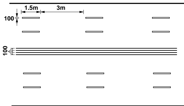
Figure 29:3: Double solid line for a two lane road
