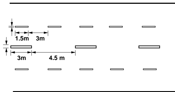
Figure 29:2: Center line and lane marking for a four lane road
