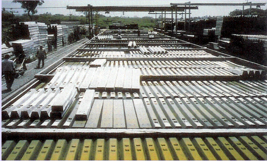
Figure 1-2.6 Linearly prestressed railway sleepers
